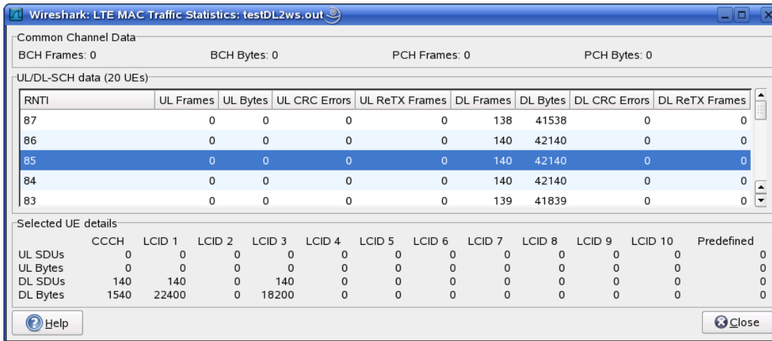
Figure 83. The “LTE MAC Traffic Statistics” window
